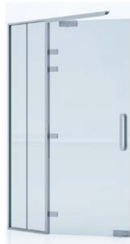
K-LITE 45 Glazing with I Joint and K-LITE 45 Door Frame.
